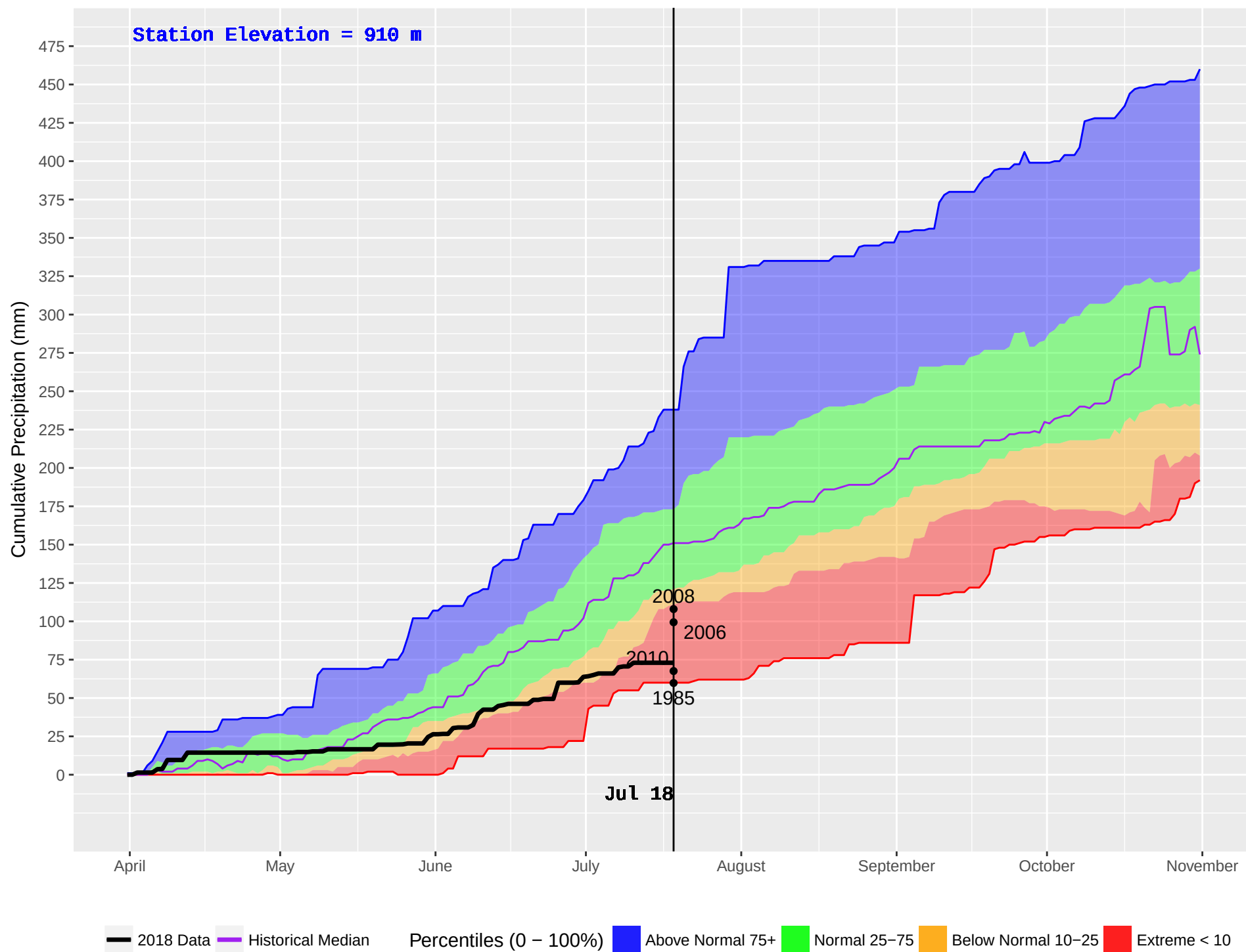
NAZKO (211) : Historical (1981–2016) and Current (2018) Daily Cumulative Precipitation
