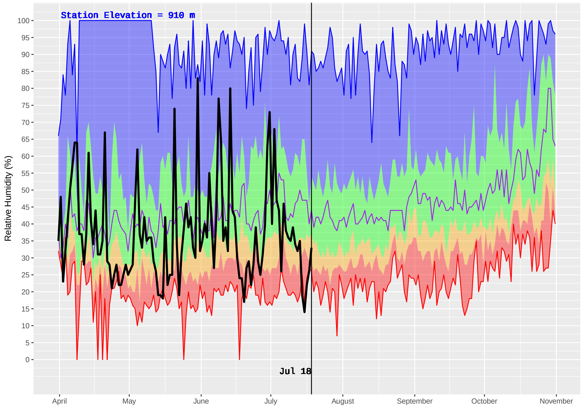
NAZKO (211) : Historical (1981–2016) and Current (2018) Daily Relative Humidity
