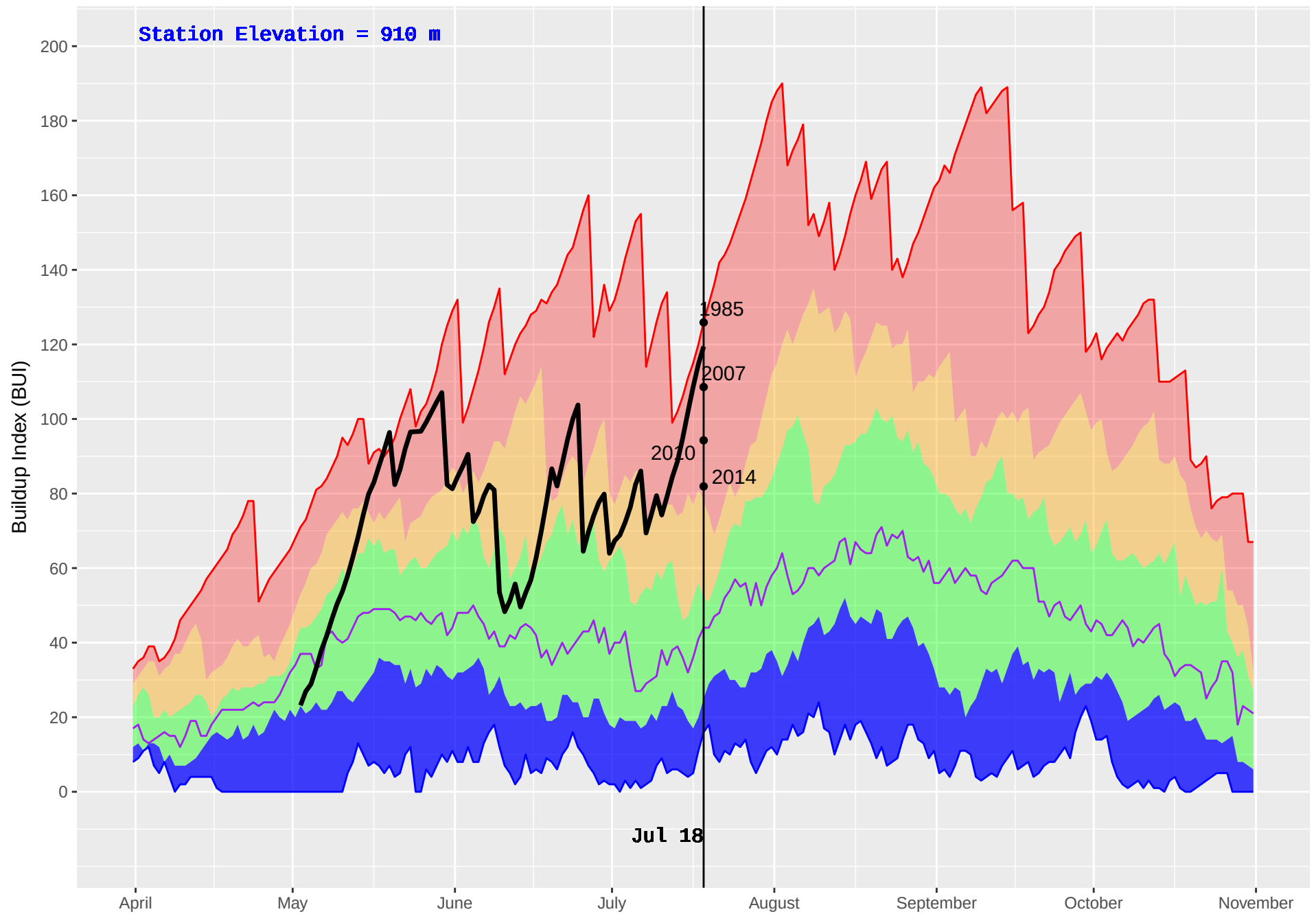
NAZKO (211) : Historical (1981–2016) and Current (2018) Daily Buildup Index (BUI)
