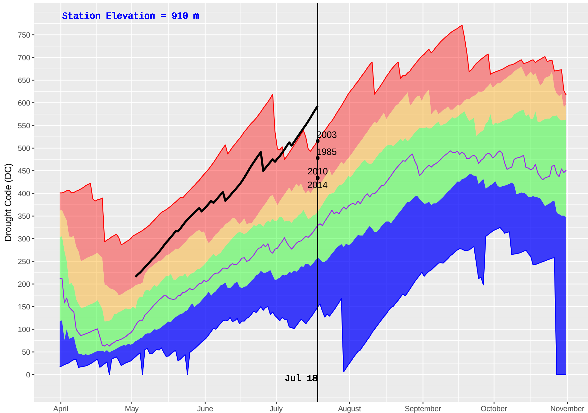
NAZKO (211) : Historical (1981–2016) and Current (2018) Daily Drought Code (DC)
