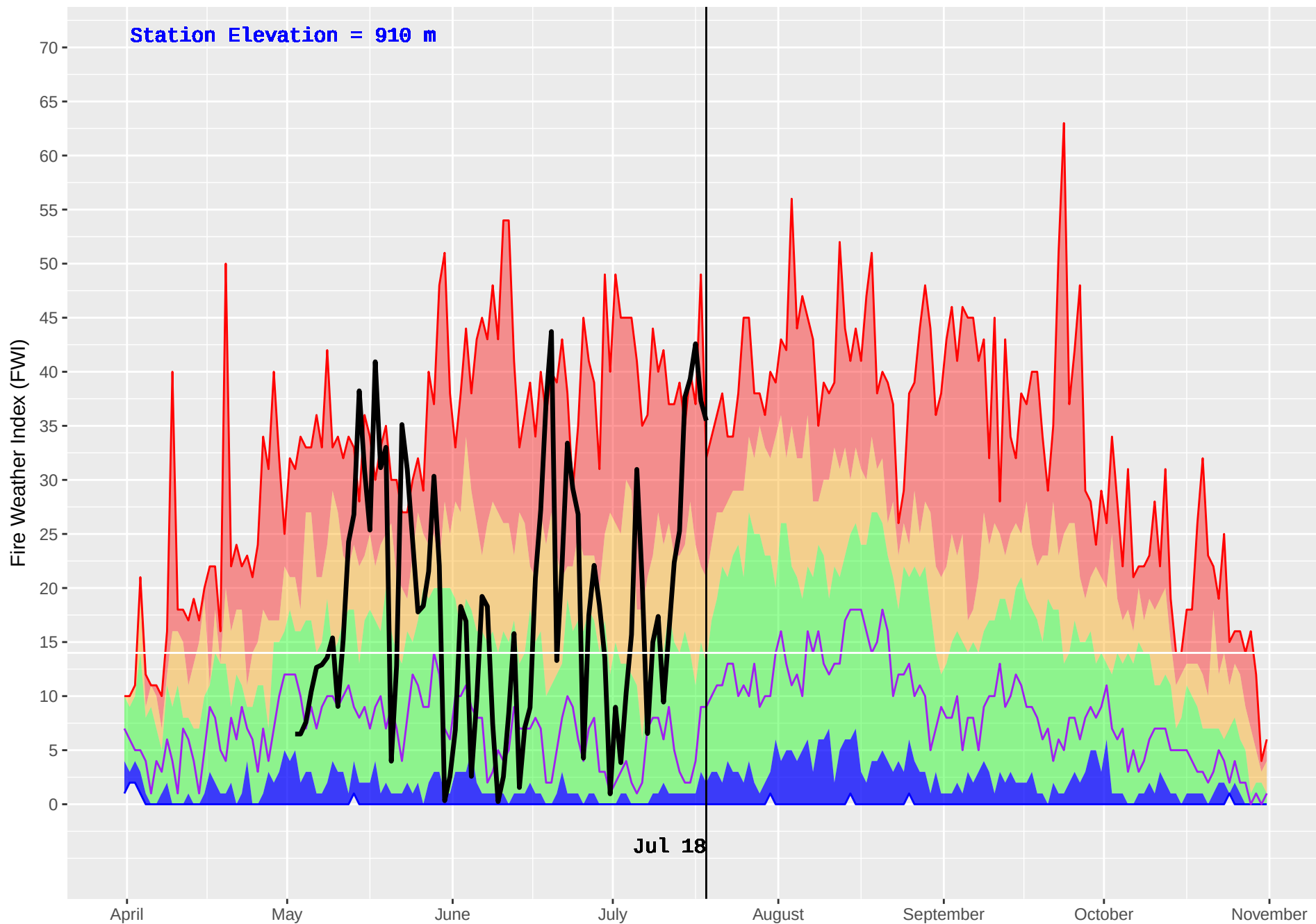
NAZKO (211) : Historical (1981–2016) and Current (2018) Daily Fire Weather Index (FWI)
