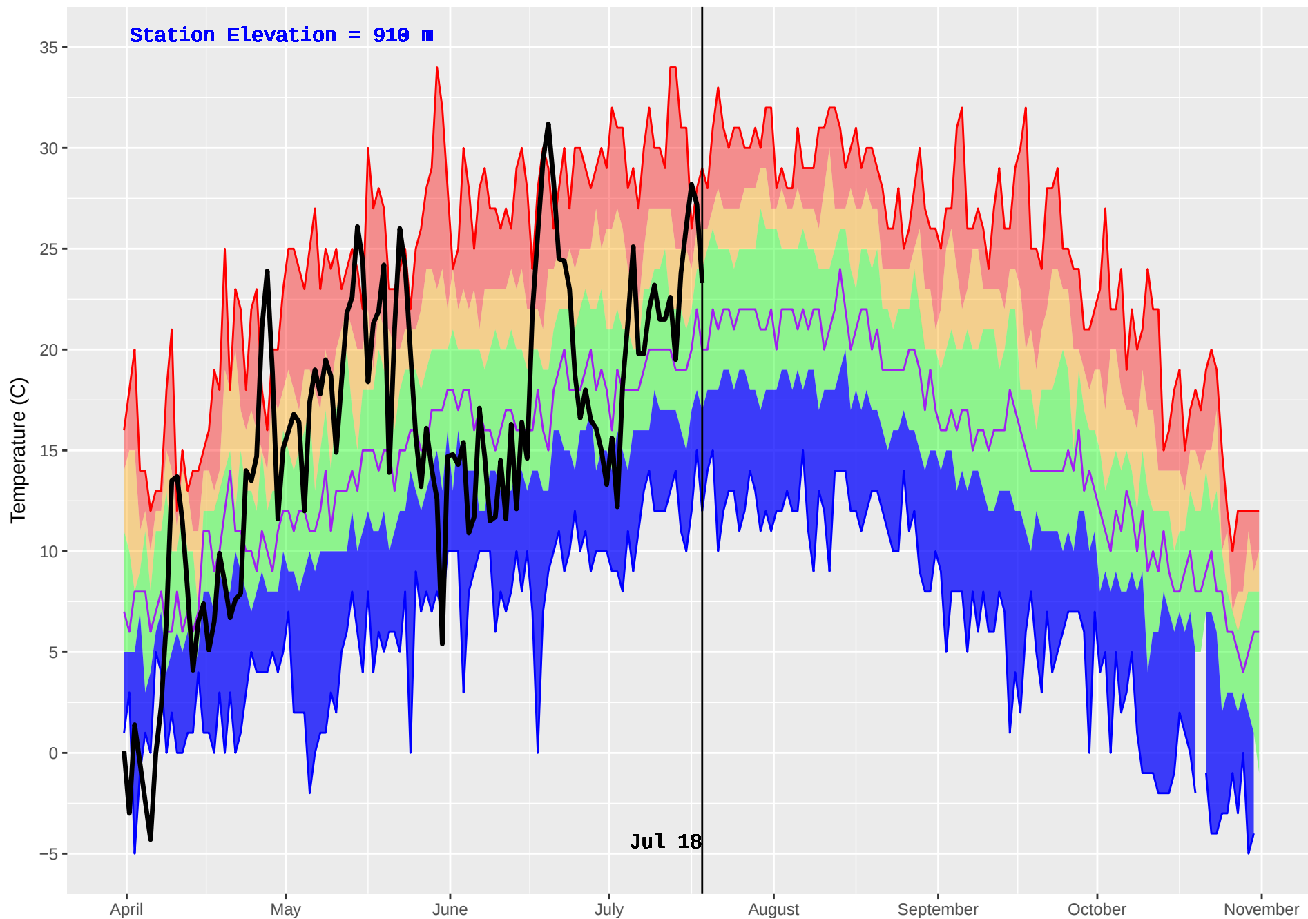
NAZKO (211) : Historical (1981–2016) and Current (2018) Daily Temperature
