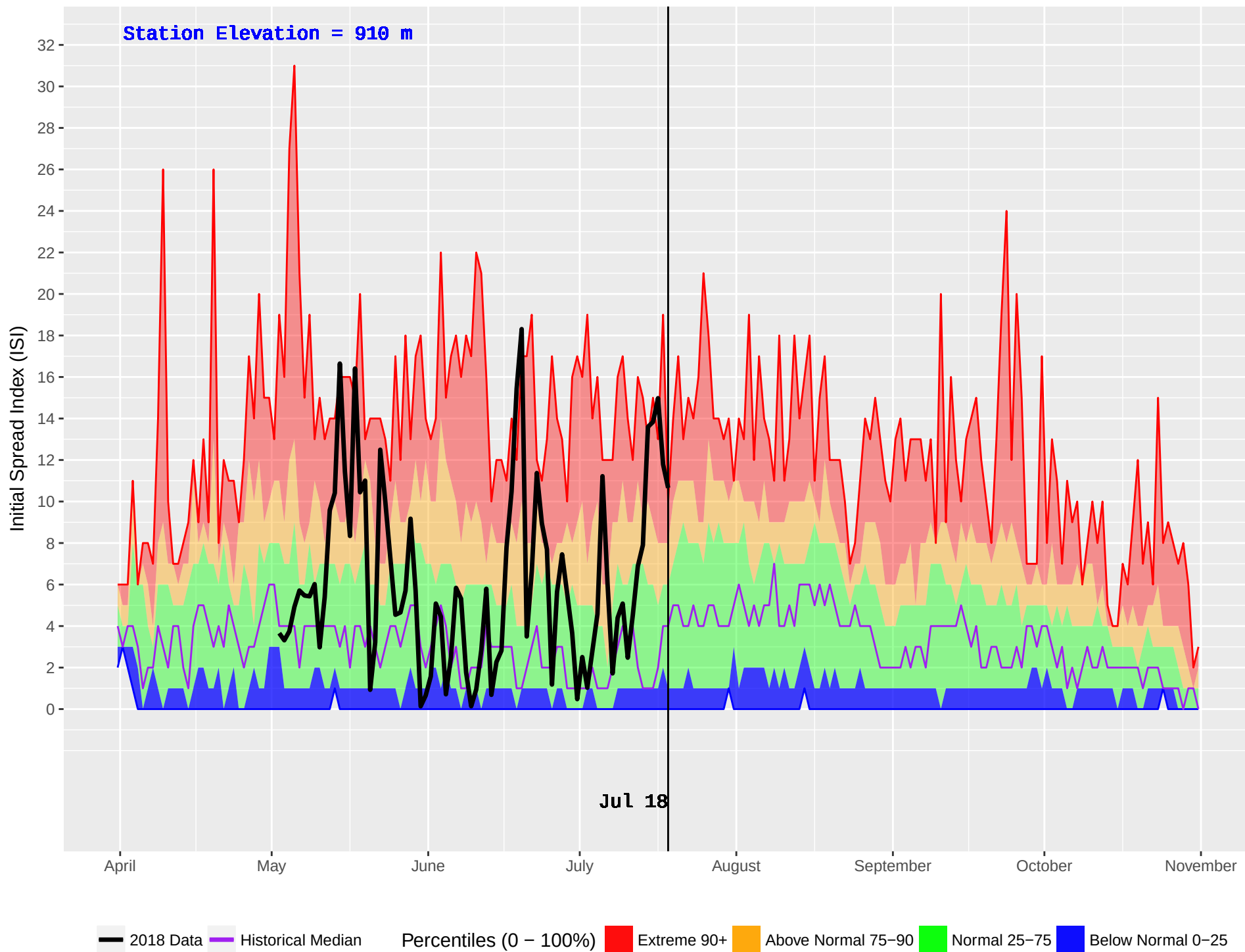
NAZKO (211) : Historical (1981–2016) and Current (2018) Daily Initial Spread Index (ISI)
