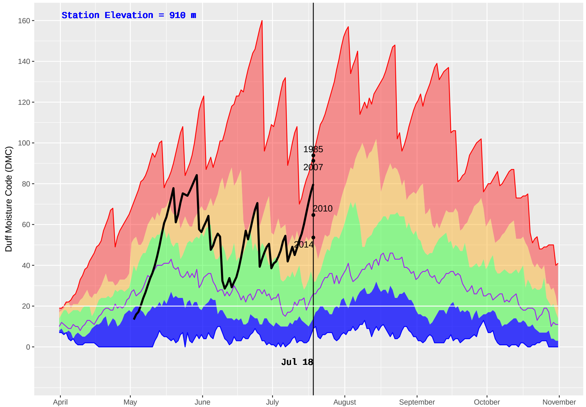
NAZKO (211) : Historical (1981–2016) and Current (2018) Daily Duff Moisture Code (DMC)
