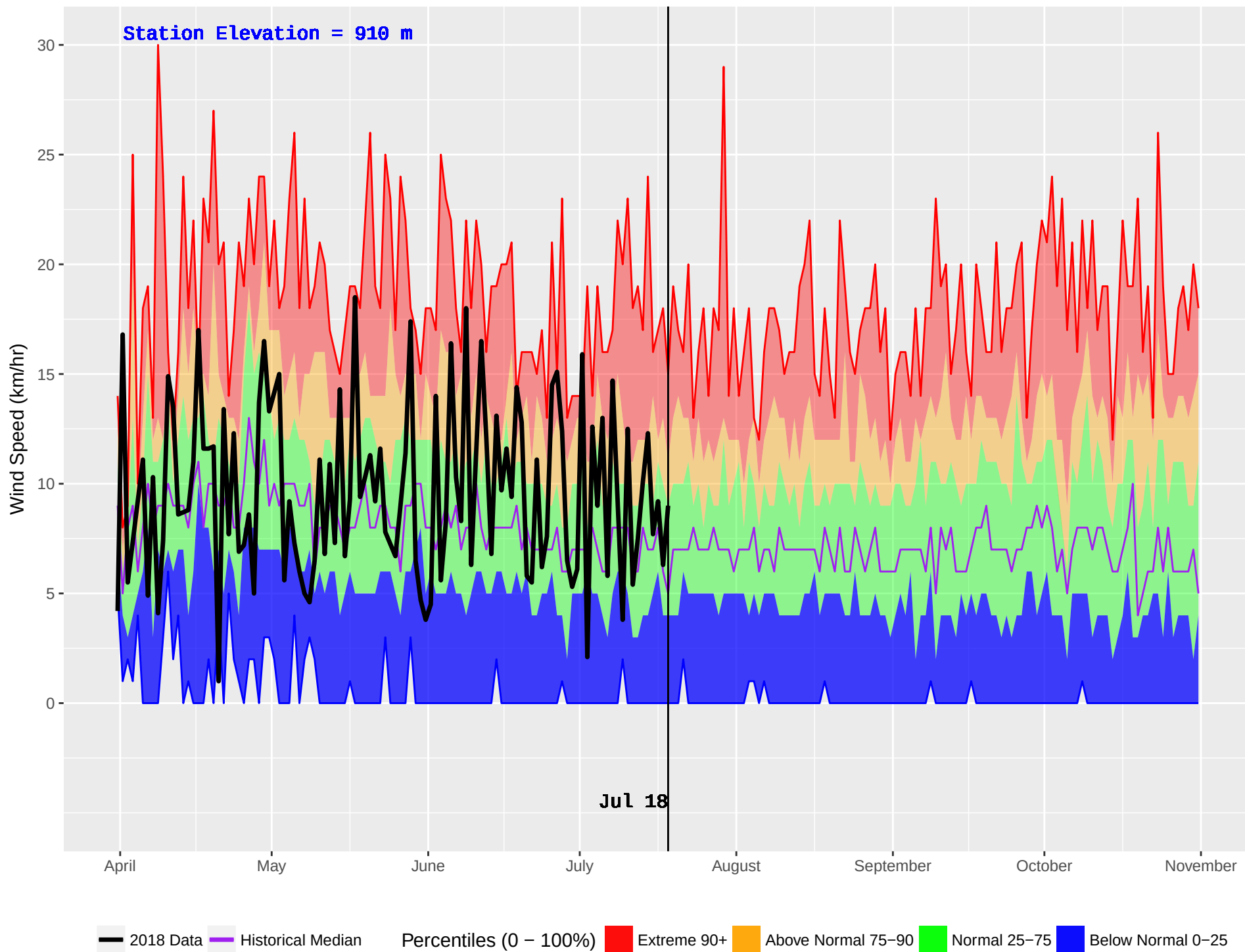
NAZKO (211) : Historical (1981–2016) and Current (2018) Daily Wind Speed
